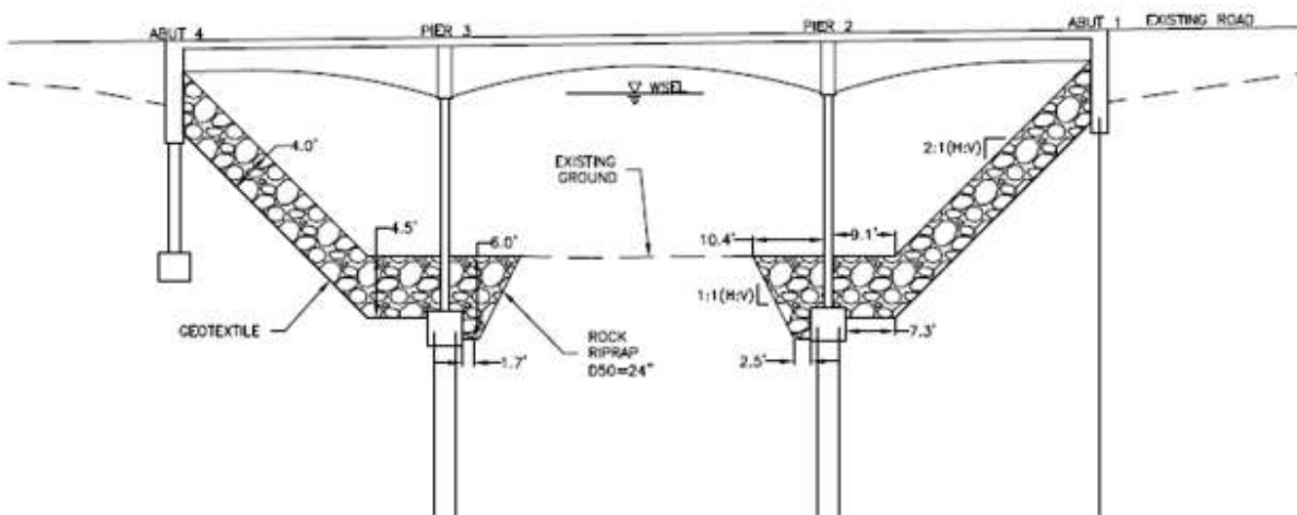
Figure 6. Cross-sectional view of Bridge B-16-FT with recommended hydraulic scour countermeasures
