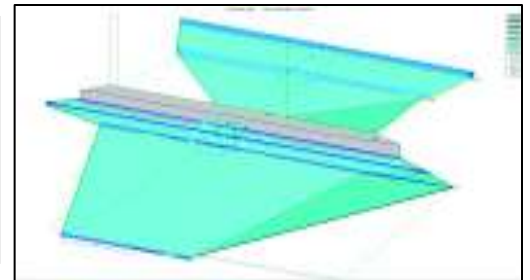
Figure 2 (Left). Water surface profile showing the 10, 50, 100 and 500-year flows Figure 3 (Right). 3D Plot of the reach around structure C-09-AR
