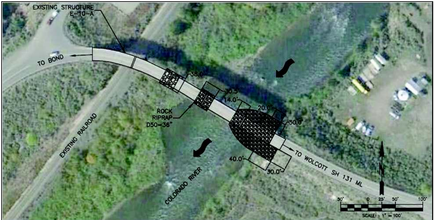
Figure 5. Plan view of Bridge E-10-A with recommended hydraulic scour countermeasure locations
